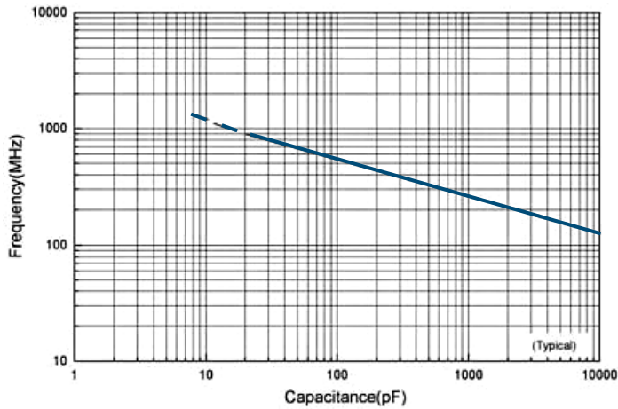
Resonance vs.Capacitance
